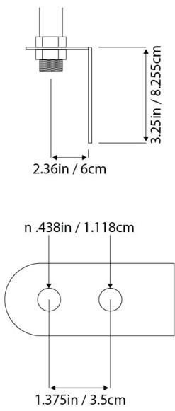
Mounting Bracket:
